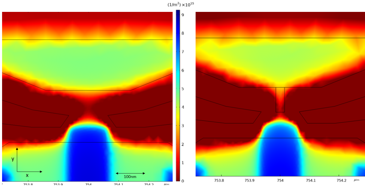
Figure 3.11: 2D maps of electron density at the surface of the 2DEG. For the left we have the device without the protrusion, and for the right we have the device with the protrusion. This map is for values of V_{\text{helper}} = 0V and V_{\text{QPC}} = -1.38V for the right figure, and V_{\text{helper}} = 0V and V_{\text{QPC}} = -0.64V for the left figure. We consider this a intermediate QPC voltage for both devices, in relation to the pinch off voltage
