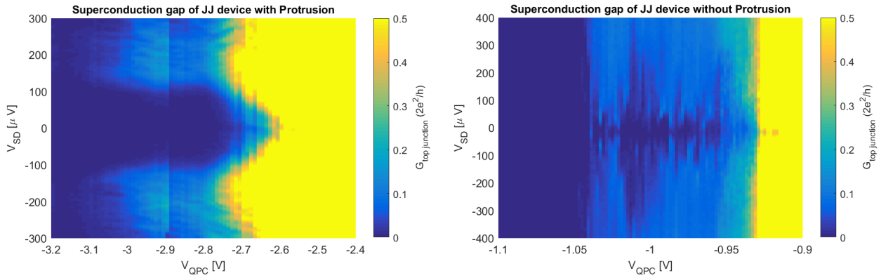
Figure 3.9: Conductance map as a function of V_{QPC} and V_{SD} for the Josephson junction device with protrusion(left) and without protrusion(right). For the left we see a clear superconducting gap, and for the right we do not see any hard gap
