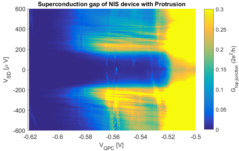
Figure 3.16: Conductance map of NIS device with protrusion, as a function of V_{\text{QPC}} and V_{\text{SD}} . For this device we see a clear superconducting gap, just as we saw figure 3.9 (left).
