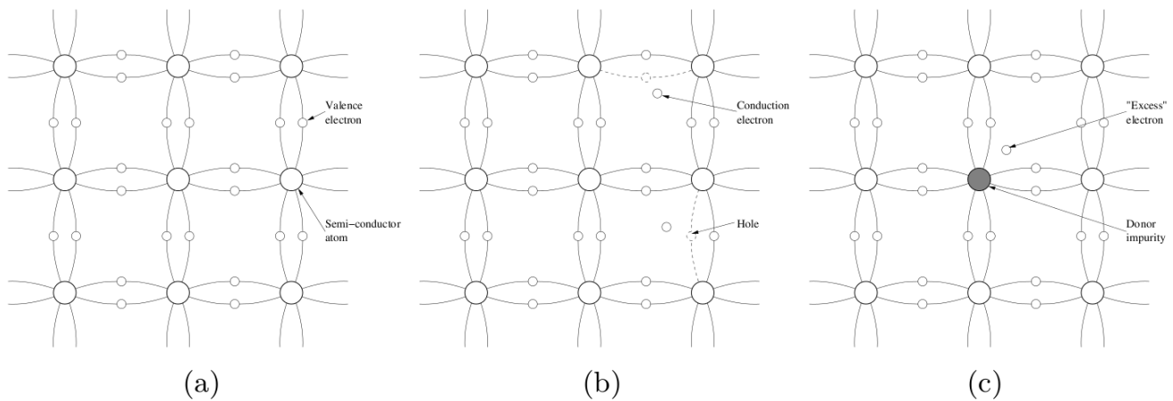
Figure 4.3: Doping [77]. Panel (a) shows semiconductor material without doping where the atoms are bound by valence electron bindings. Panel (b) illustrates the concept of a ‘hole’ left behind by a conduction electron. Finally, (c) shows doped semiconductor with the impurity atom inserted in the semiconductor lattice.
