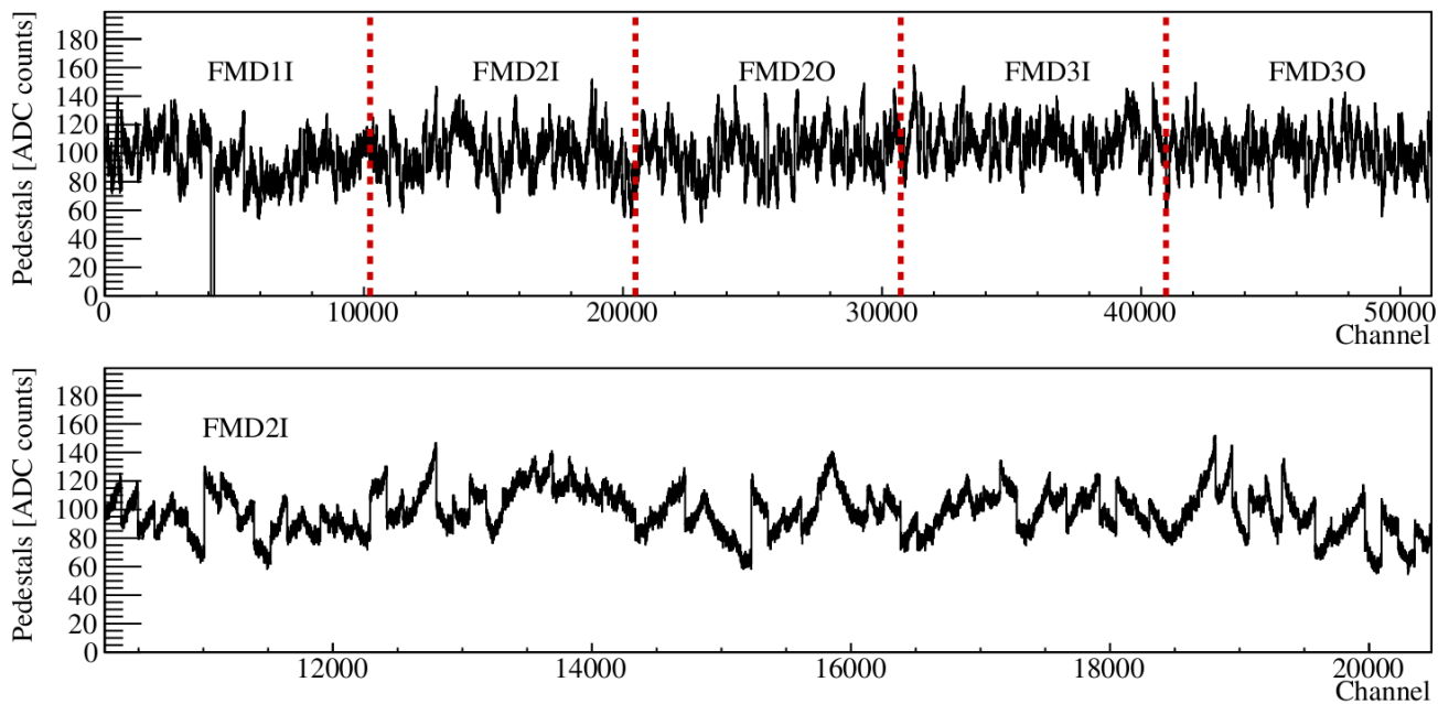
Figure 5.3: The pedestals valid for run 138225 shown for all channels in the FMD.
