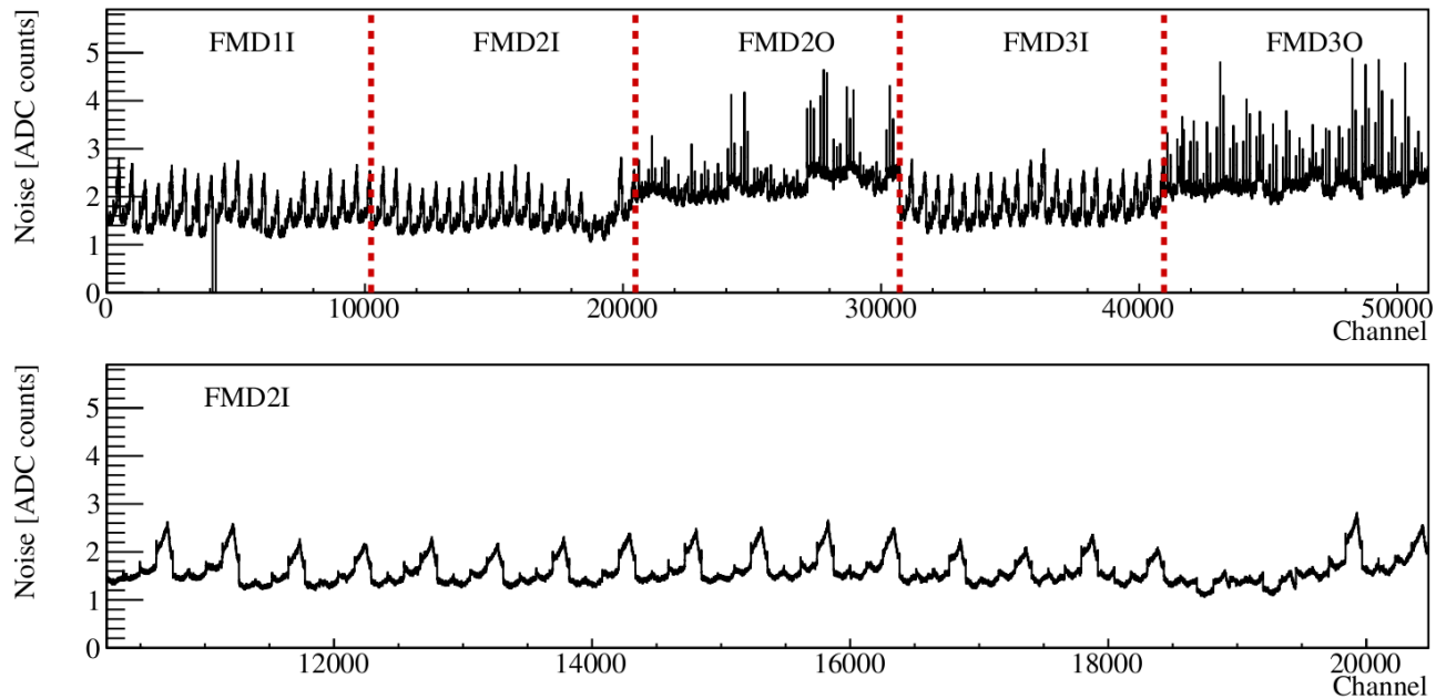
Figure 5.4: The measured noise valid for run 138225 shown for all channels in the FMD.
