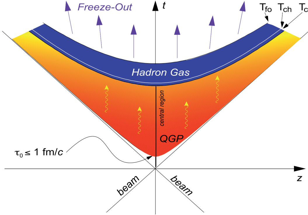
Figure 1.10: The Bjorken space-time diagram [4]. The (z, t) hyperbolae mark the boundaries between the different phases.
