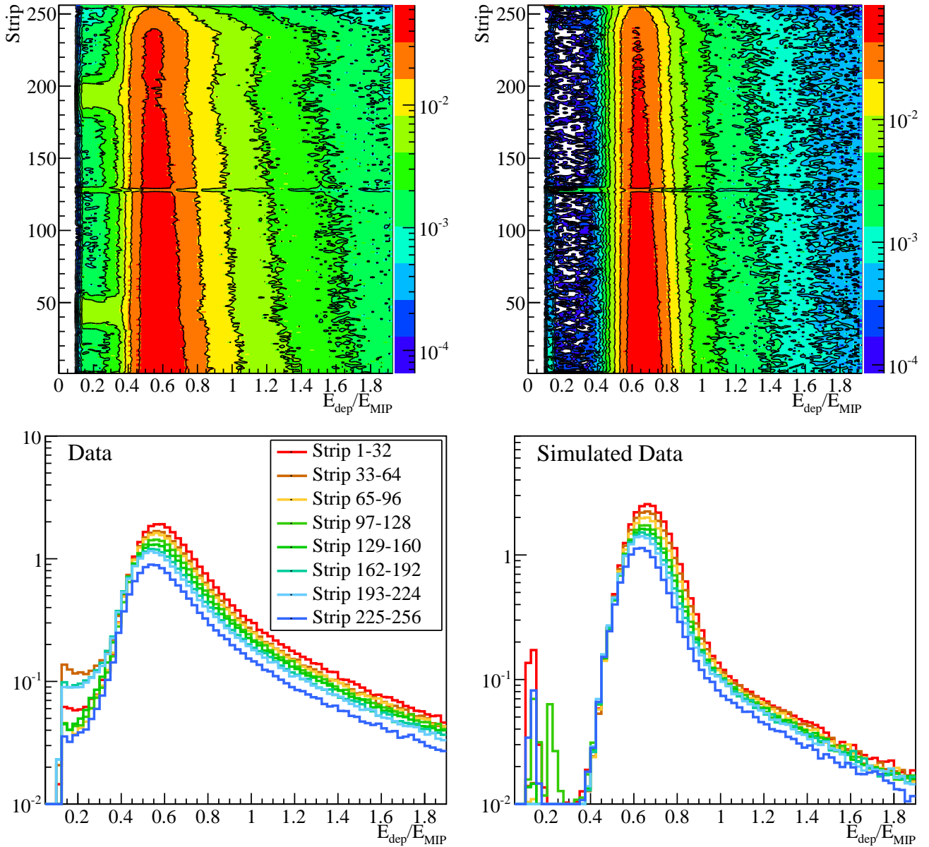
Figure F.1: The top panels show the single strip energy signal versus strip in FMD20 in \sqrt{s} = 900 GeV p+p physics data (left) and simulated data (right). While the general features are similar a structure at low energies ( E_{dep}/E_{MIP} \sim 0.2 ) is observed in physics data which is not present in the simulated data. This is also evident from the lower panels which show the projections of groups of 32 strips. Apart from the observed structure it is clearly seen that the low energy tail is much more pronounced in physics data than in simulated data. The band structure at strip \sim 128 is understood as a consequence of dead channels.
