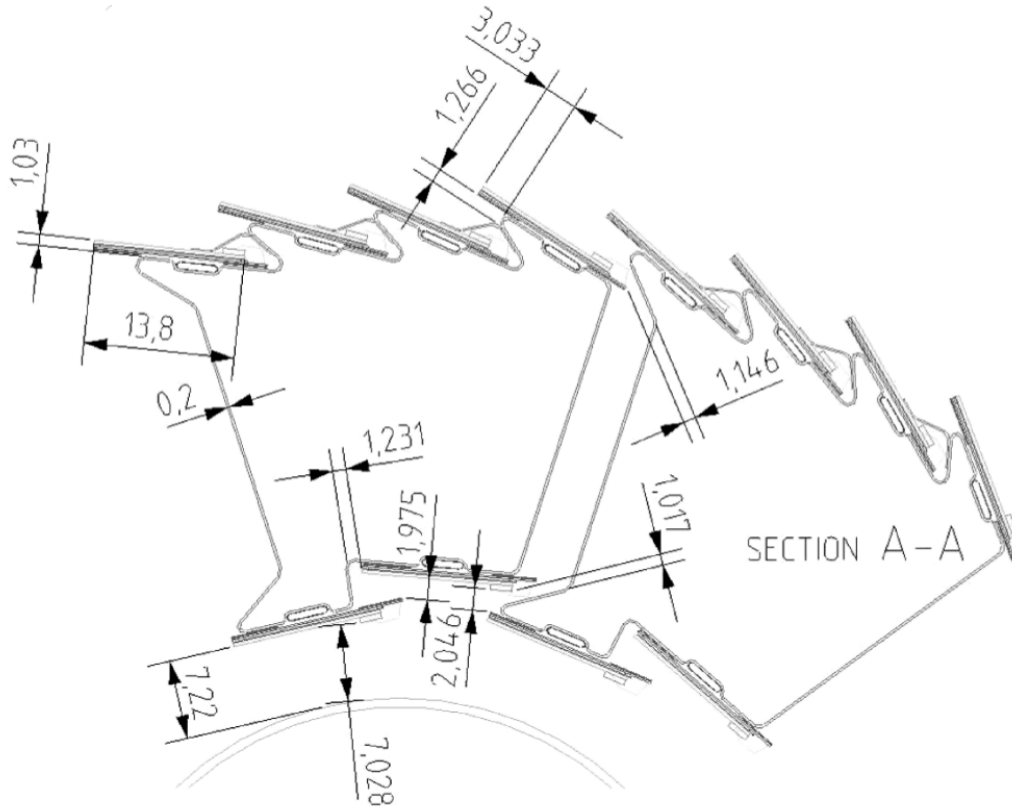
Figure 5.6: A cut through the SPD showing the positions of the Si-pixel (half)staves [79]. The beam pipe is visible at the bottom. Note that the gap between the SPD and the beam pipe is only \sim 7 mm so the SPD almost literally sits on top of the beam pipe.
