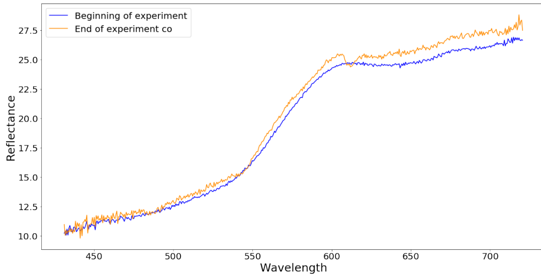
Figure 32: Spectra showing the reflectance of the soil samples with 50 % perchlorates, where end data has been corrected.
