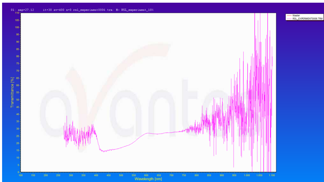
Figure 7: Raw data spectra showing the reflectance of the soil samples with 10 % perchlorates. Please note, that even though the image says transmittance, it was the reflectance that was measured.
