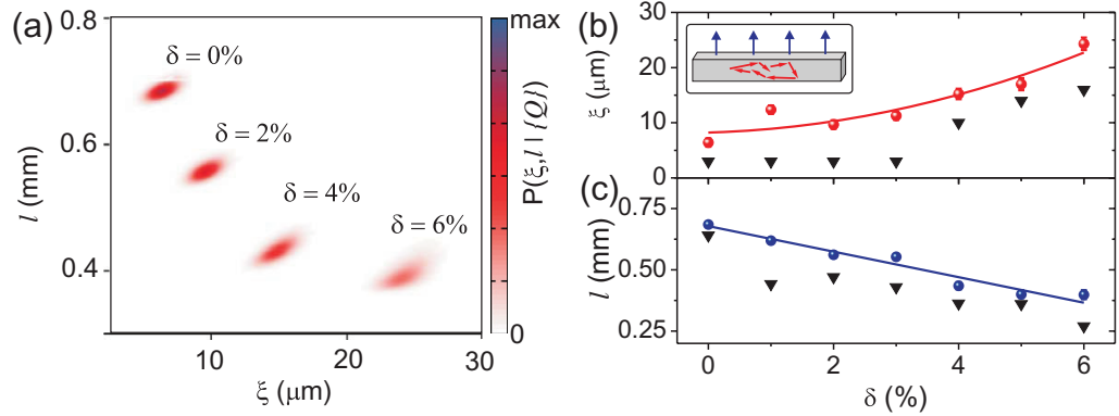
Figure 3. (a) Conditional probability P(\xi, l | Q) that a disordered 1D medium with a localization length \xi and average loss length l can be described by the measured Q factor distributions, plotted as a function of \xi and l and for various degrees of disorder. (b) Localization length versus degree of disorder. The red circles are obtained from the data in panel (a) by locating the value where the probability P(\xi, l | Q) is largest. The black triangles are obtained from P(\xi, \mu_1, \sigma_1 | Q) where a distribution of loss lengths were included. Inset: sketch of the light scattering processes (red arrows) and out-of-plane scattering (blue arrows). (c) Blue circles (black triangles) are the average loss lengths extracted from P(\xi, l | Q) ( P(\xi, \mu_1, \sigma_1 | Q) ). The solid curves in (b) and (c) are guides to the eye.
