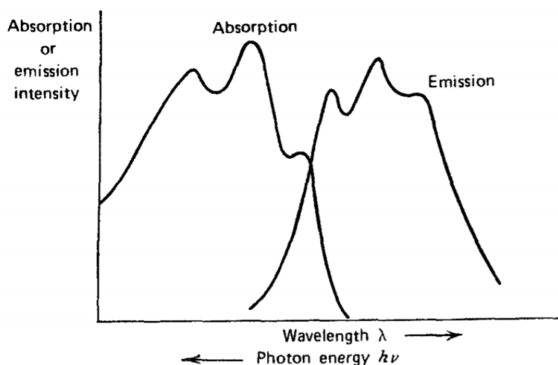
Figure 4.2: Illustration of the Stokes shift for a typical organic scintillator: difference in optical absorption and emission spectra [47].
