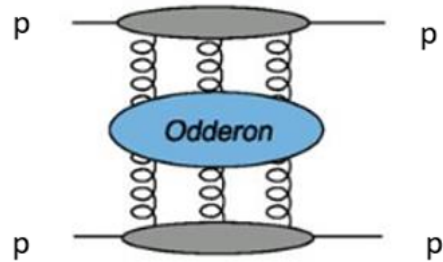
Figure 2.12: Odderon exchange.
