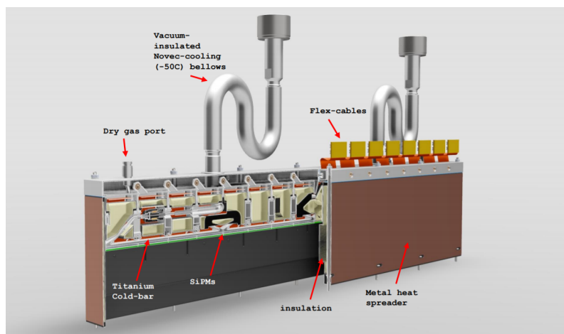
Figure 6.15: Cross sectional view of the cold box: Novec cooling and dry gas flushing [72].
