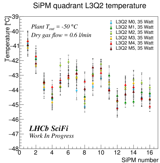
Figure A.14: Temperature dispersion comparison for modules of quadrant L3Q2.
