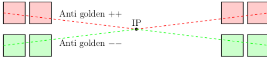
Figure 9.7: The two antigolden arms: ++ refers to upper detectors and – to lower detectors [20].
