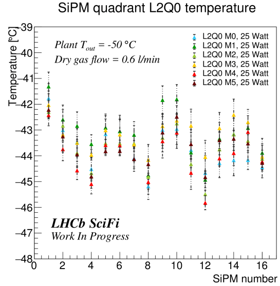
Figure A.12: Temperature dispersion comparison for modules of quadrant L2Q0.
