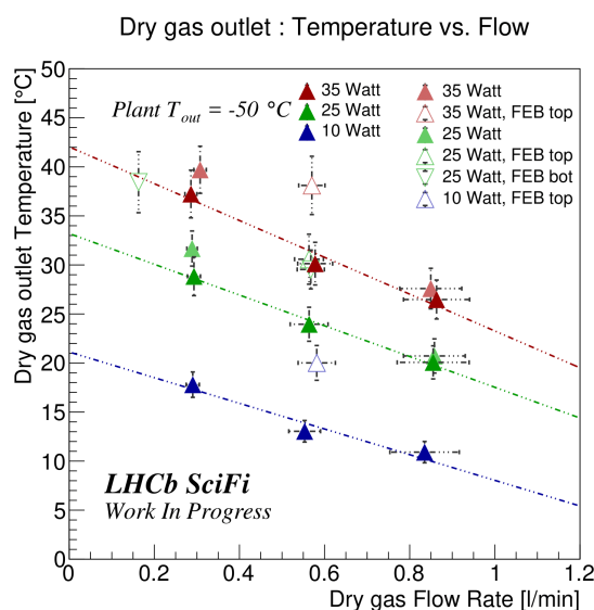
Figure 7.14: The dry gas outlet temperature measured as a function of the dry gas flow rate under three different heating settings.
