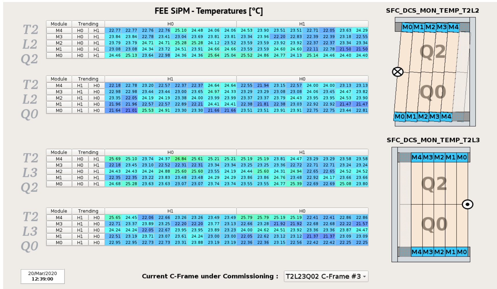
Figure 7.7: Tabulated SiPM temperatures for a c-frame, arranged per module.
