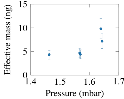
Figure 1.16: Effective masses of defect modes. We determine the effective masses from the maximum of displacement maps shown in Figure 1.15. The dashed line shows the calculated effective mass of a square membrane, whose fundamental mode has the same frequency as mode A.
