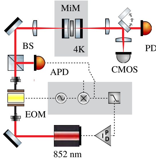
Figure 2.5: Illustration of the optical setup around the MiM system. We couple laser light at a wavelength of \lambda = 852 nm into the MiM cavity. The latter is placed in a cryostat at a temperature of T = 4.2 K. Reflected light from the cavity is detected by an APD whose signal is used to stabilize the laser frequency to the cavity using slope locking or the PDH technique. In transmission we can directly detect the light with a photodetector (PD) or insert a mirror on a flip-mount to image the membrane onto a CMOS camera.
