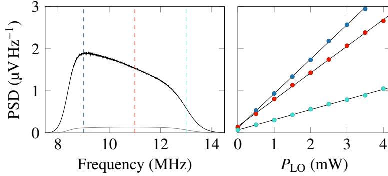
Figure 2.15: Response of the balanced heterodyne detector. Left: Averaged PSD from a SN measurement (black line) at an optical power of P_{LO} = 2.05 mW balanced between the two photodiodes of BAC3. The gray line shows the electronic noise of the detector and the colored dashed lines indicate the frequency bins at which we extract the SN level for the plot on the right. Right: SN level in the PSD versus P_{LO} for the three frequency bins indicated on the left. Dots are data points, whose color-code refer to the dashed lines, and black solid lines are linear fits.
