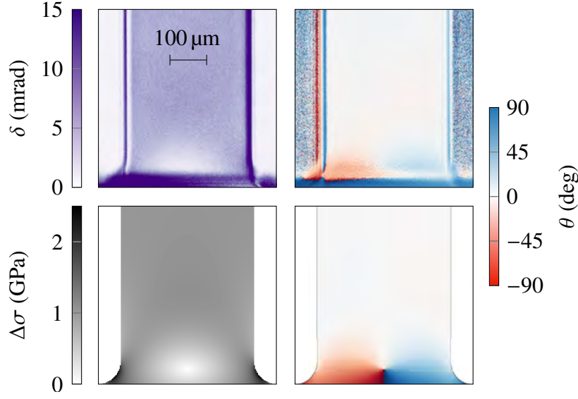
Figure 1.10: Stress analysis of a SiN ribbon. Top: Retardation \delta (left) and angle of optical axis (right) measured with our gray field polariscope at one end of a SiN ribbon with a film thickness of 210 nm. Bottom: Simulated stress anisotropy \Delta\sigma (left) and angle of principle stress \theta (right) for the same device as above. Redrawn from [2].
