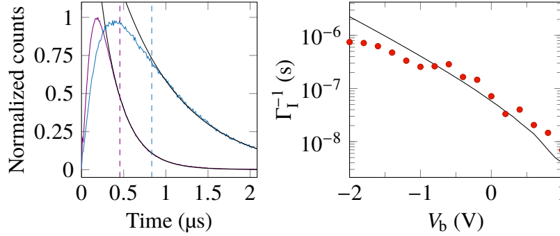
Figure 3.8: Decay dynamics of the charge carriers. Left: Time-resolved PL measurements at the indirect transition wavelength for bias voltages V_b of -2 V (blue) and -1 V (purple), where black lines are fits. Colored dashed lines indicate the start time of the fits. The photon counts are normalized to the peak value in each trace. Right: Extracted lifetimes for \Gamma_I (red dots) as a function of V_b , as well as calculated lifetimes of the indirect transition (black). Redrawn from [4].
